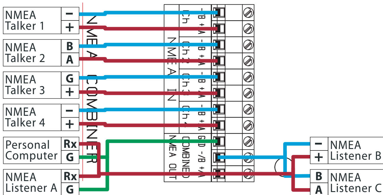
Figure 2 – NMEA 0183 connections
