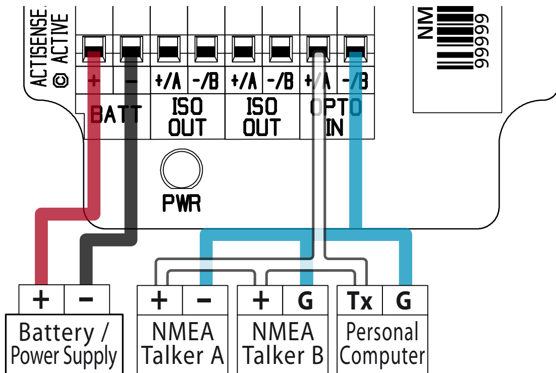
Figure 2 – Input connections
